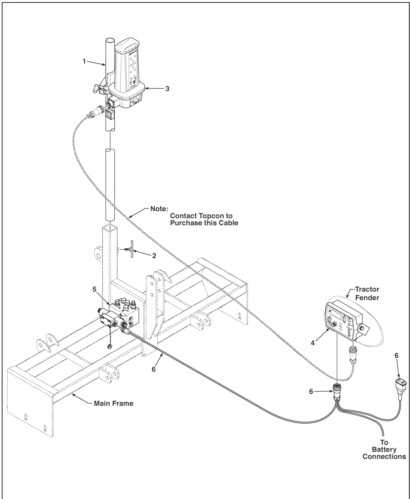
Figure 17. Laser Controls and Related Parts - Topcon System Five and LS-B4 BSN2096
