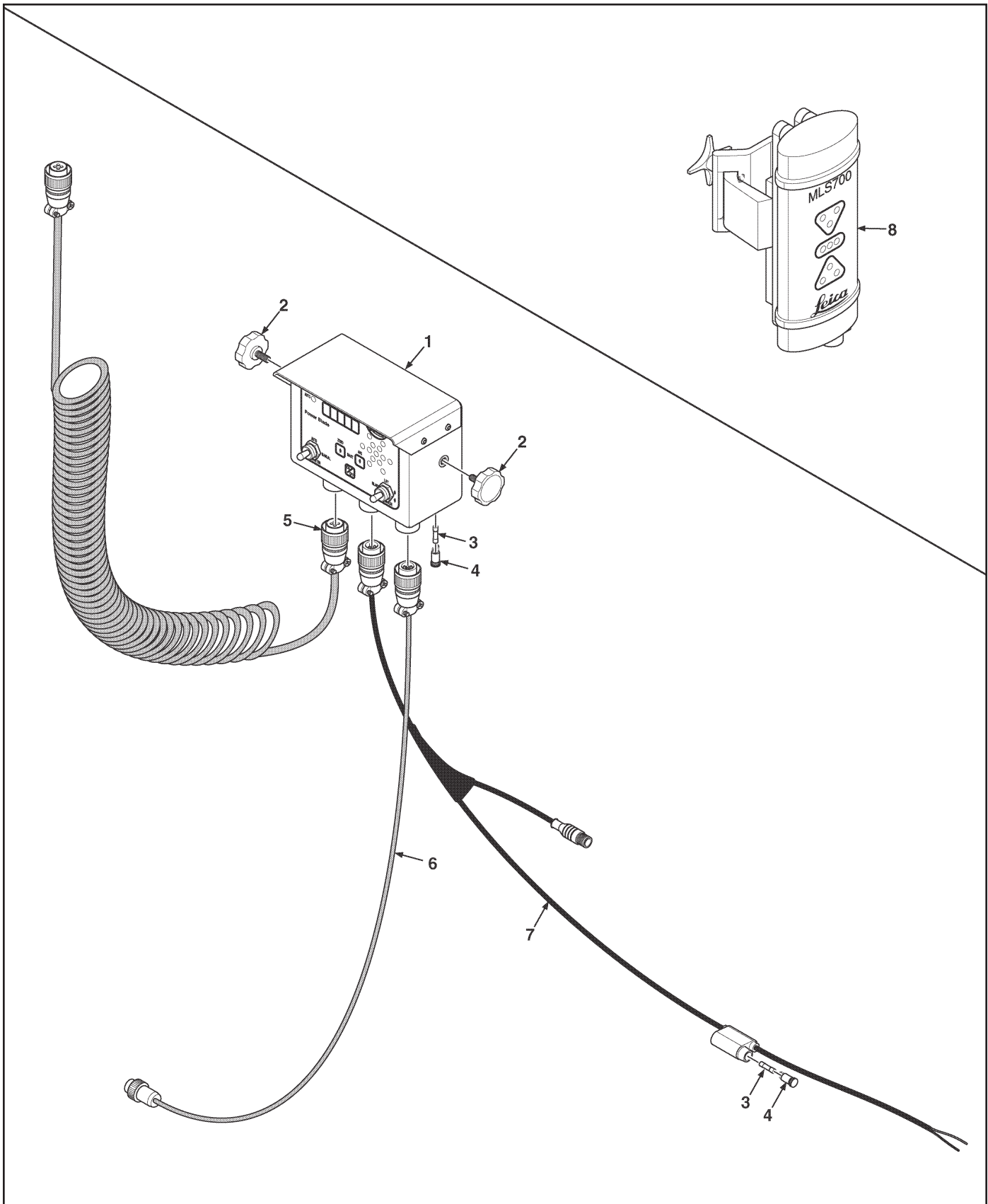
Figure 15. Control Panel, Receiver, Cables - Leica MCP700
