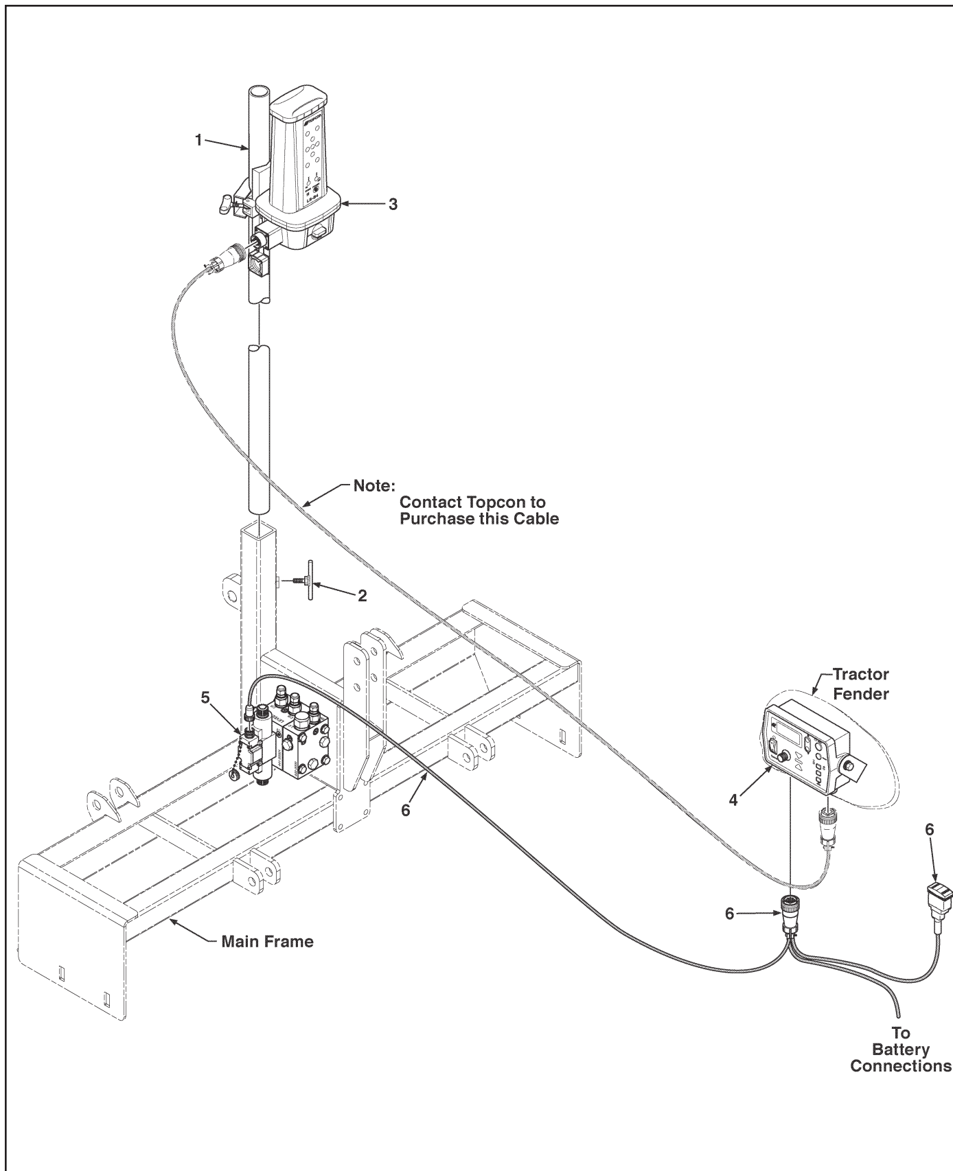
Figure 16. Laser Controls and Related Parts - Topcon System Five and LS-B4 ASN2095
