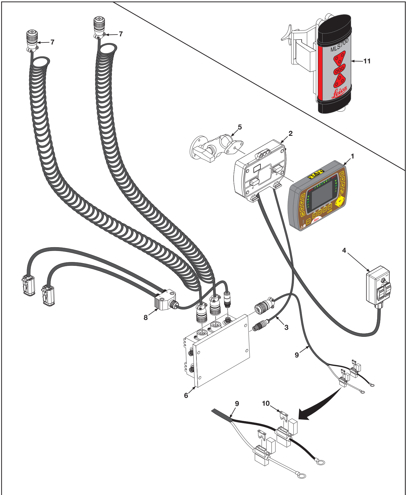
Figure 10. Control Panel, Laser Receiver 360°, Cables - Leica iCON
