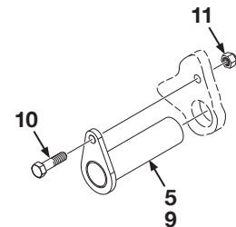
Typical Pivot and Link Pins Installation 9 Places
