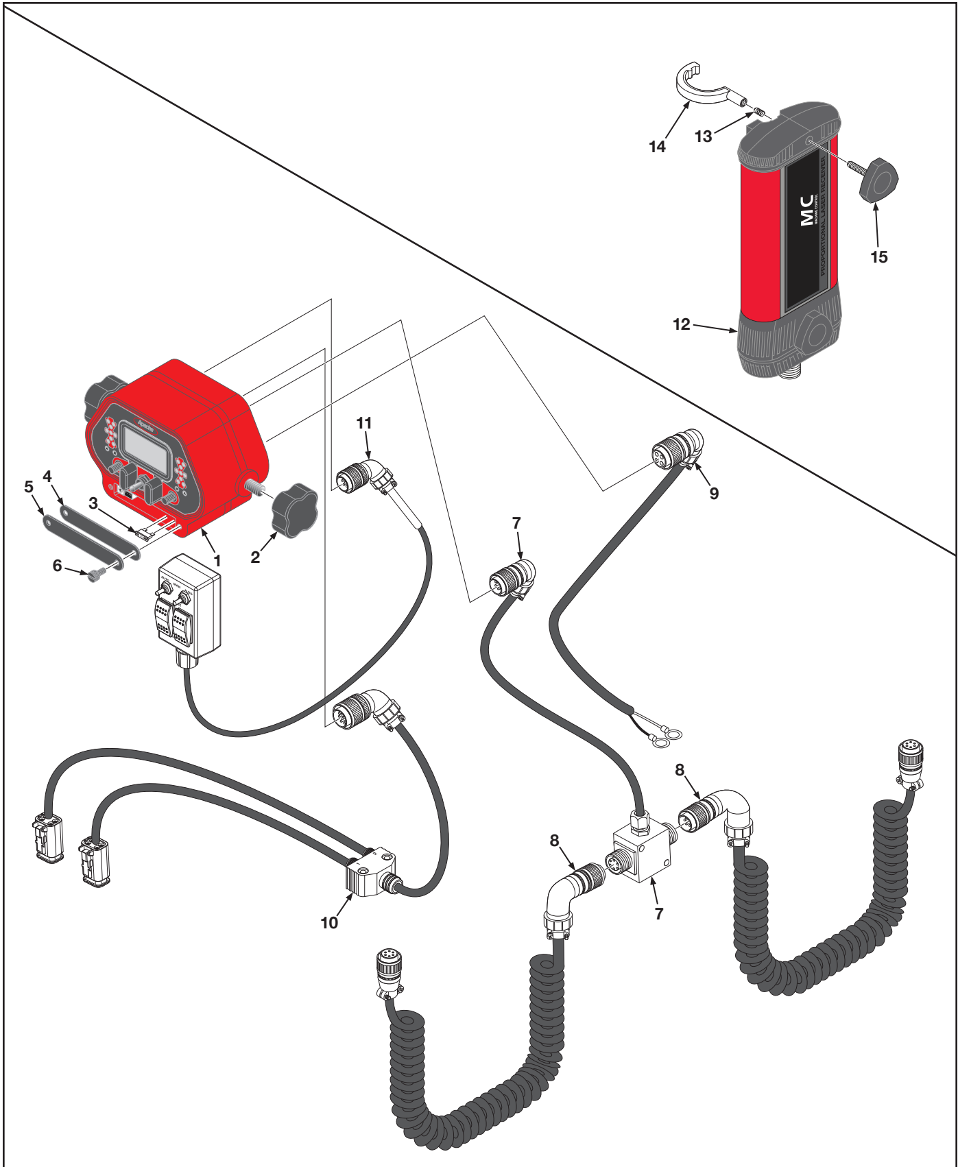
Figure 8. Control Panel, Laser Receiver 360°, Cables - Apache/Spectra
