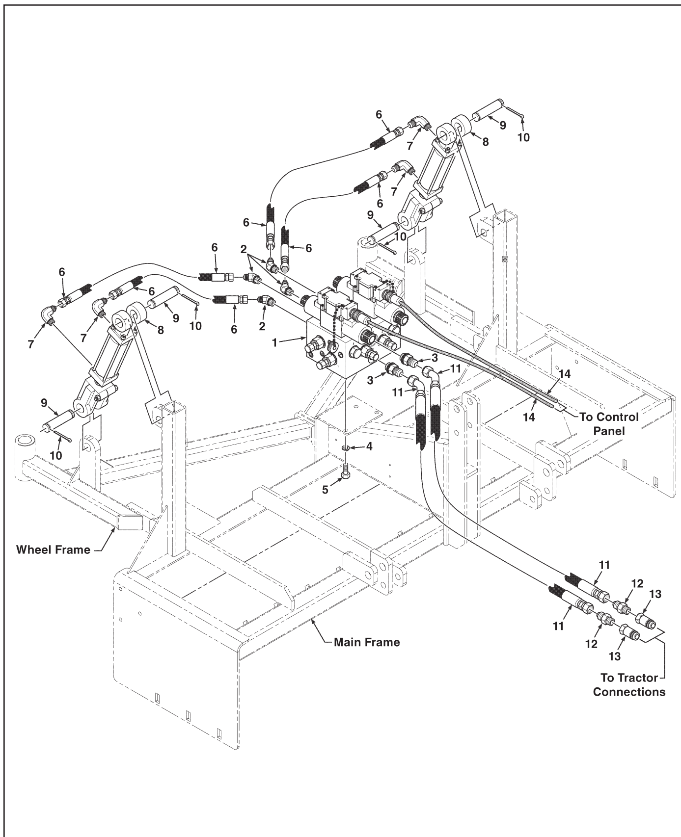
Figure 6. Hydraulics With Optional Valve Assembly - BSN1440 - ASN1259
