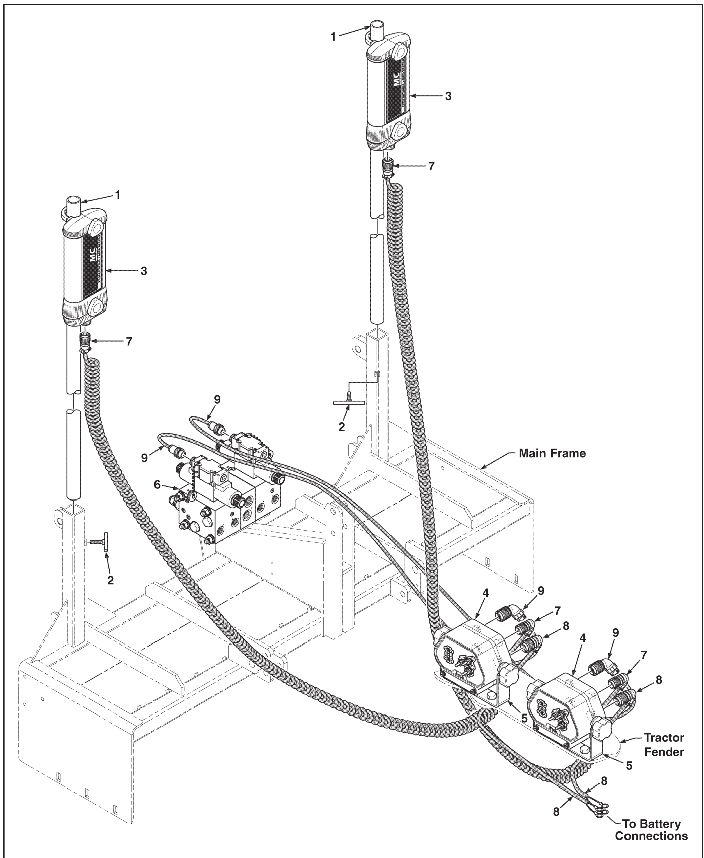
Figure 11. Laser Controls and Related Parts Apache CB26 - ASN1439
