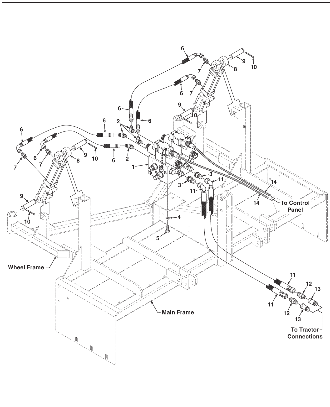
Figure 7. Hydraulics With Optional Valve Assembly - BSN1260
