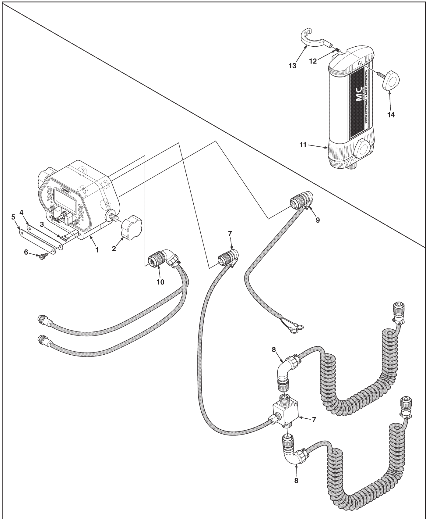
Figure 13. Control Panel CB52, Receiver, Cables and Related Parts - ASN1439
