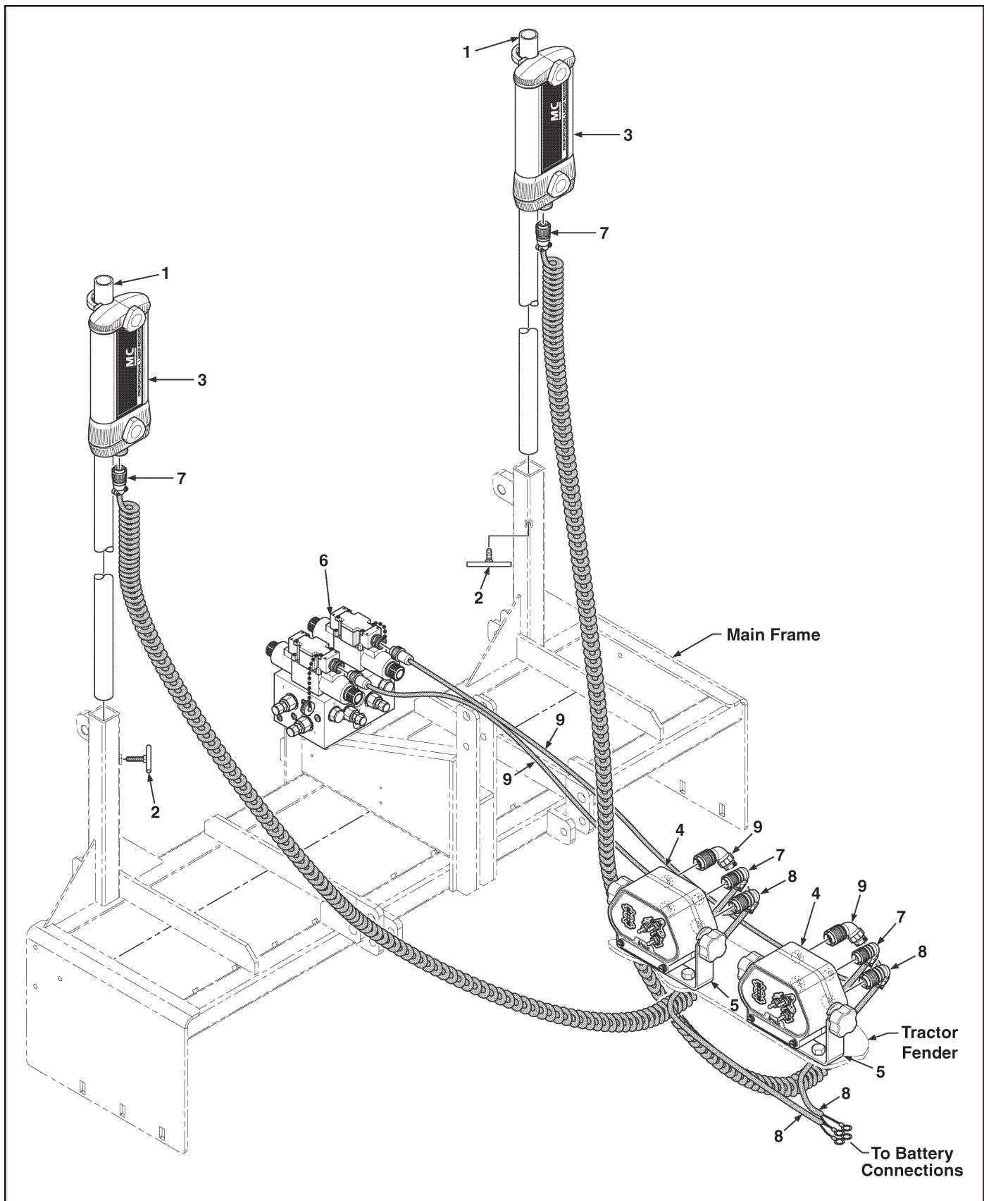
Figure 12. Laser Controls and Related Parts Apache CB26 - BSN1440
