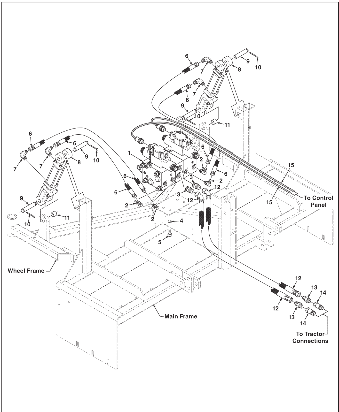
Figure 5. Hydraulics With Optional Valve Assembly - ASN1439
